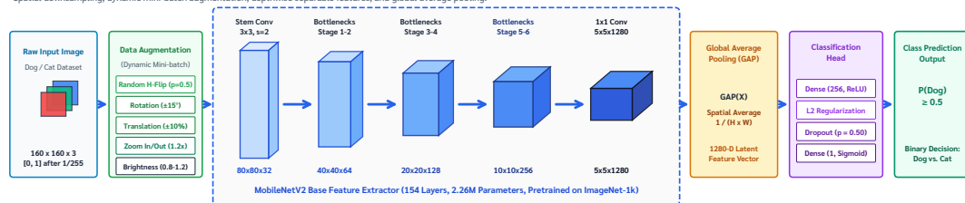
Figure 2(a): End-to-End Transfer Learning Computational & Tensor Pipeline
